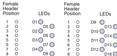
Figure 3. LED Positions
